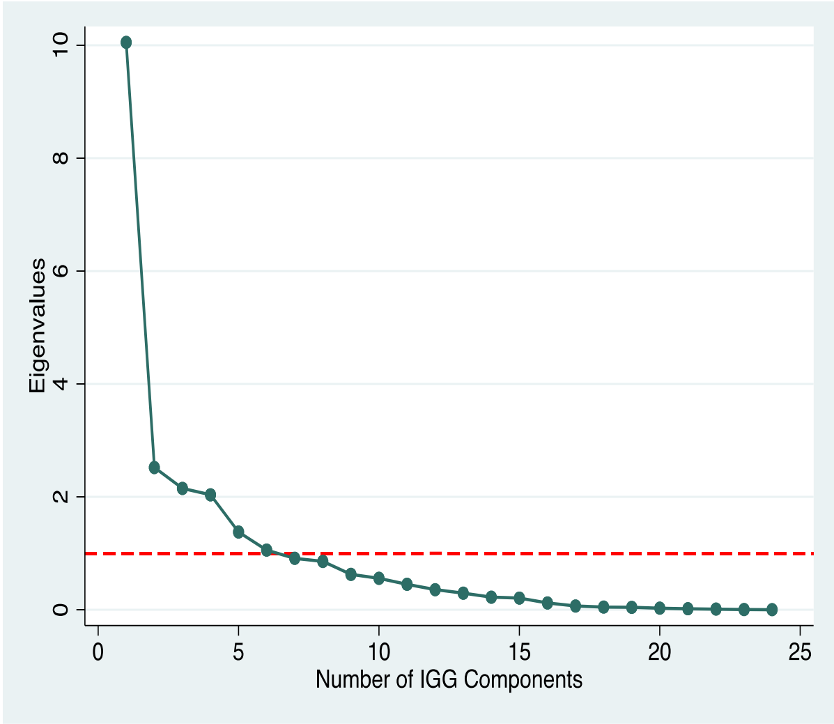
Figure A.1: Screeplot of IGG Components
