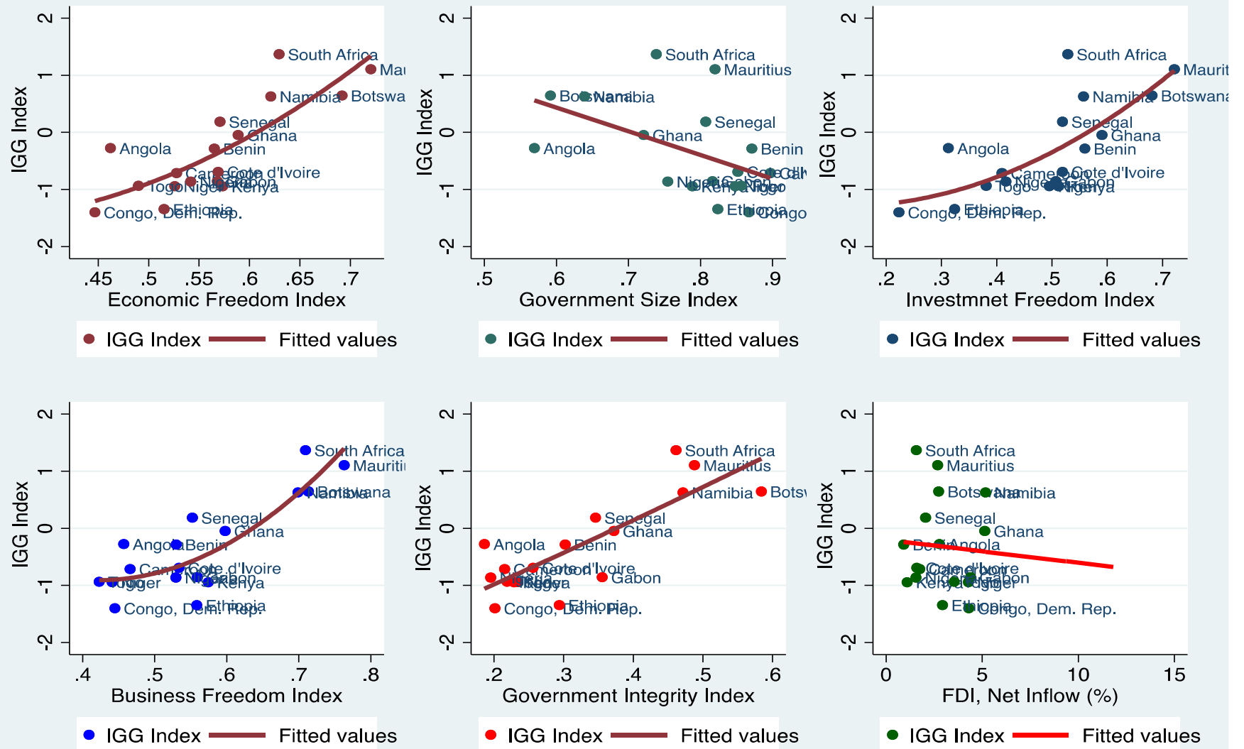
Figure 2: Relationship between FDI, economic freedom and inclusive green growth.
