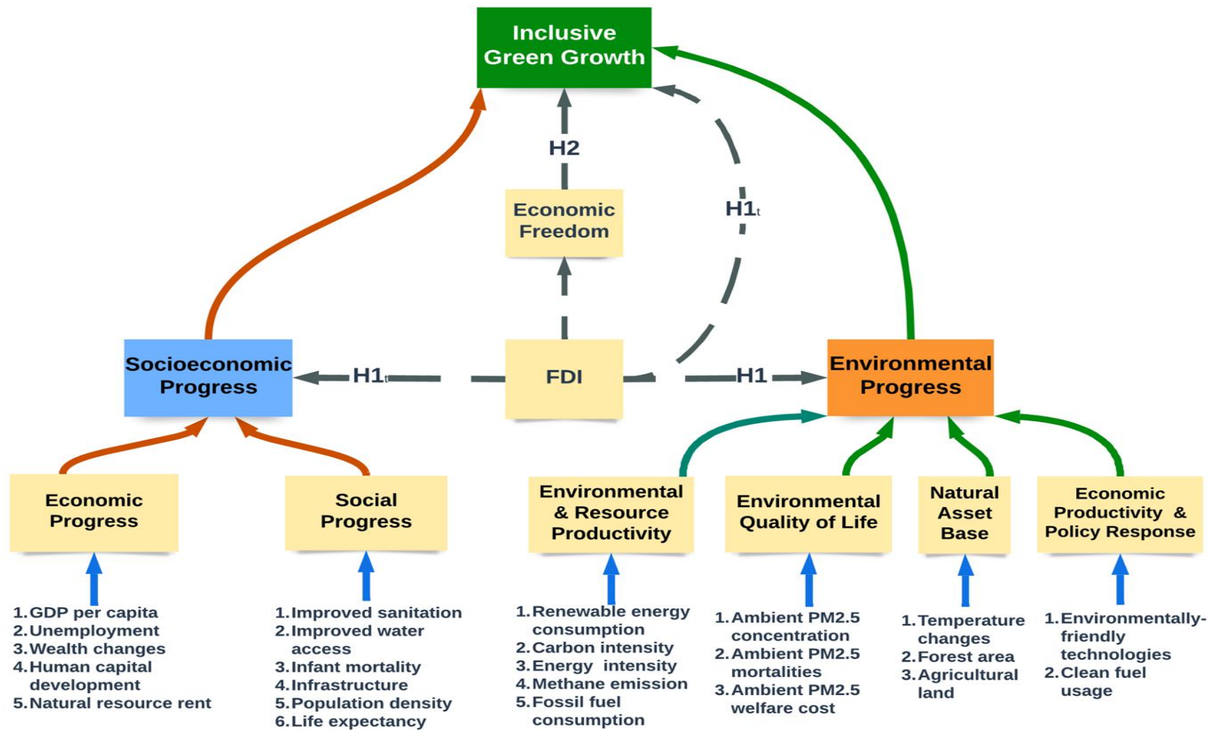
Figure 1: Analytical framework for inclusive green growth
