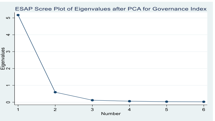
(E): East & South Asia and the Pacific (ESAP) region scree plot of Eigenvalues for Governance and ICT development indexes
