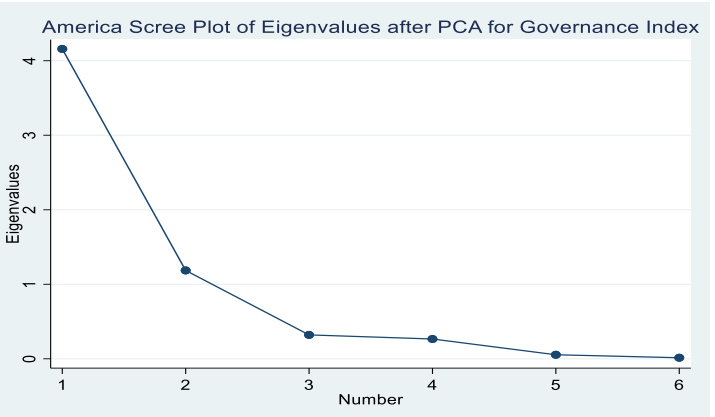
(F): America region scree plot of Eigenvalues for Governance and ICT development indexes
