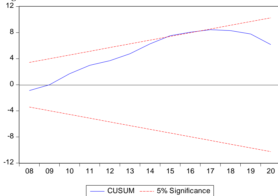
Figure 1: CUSUM
